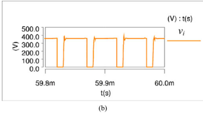
Fig. 14. Simulation results of the voltage-fed trans-qZSI considering the parasitic capacitance of the bifilar winding (constant boost control, M = 0.93 , D_{sh} = 0.2 ). (a) Input and capacitor voltages and output voltage/current. (b) Inverter dc-link voltage.
